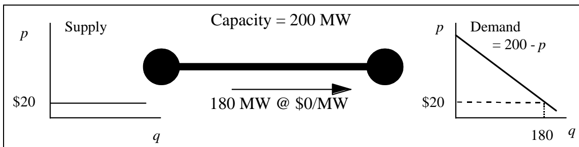
Figure 1: Efficient Dispatch
