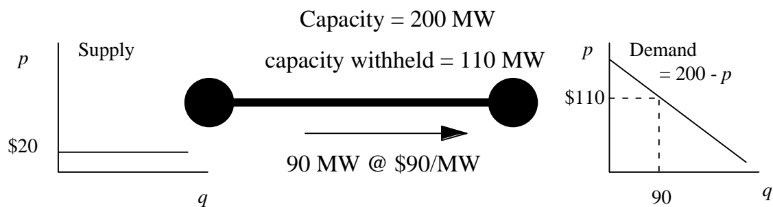
Figure 3: Transmission Monopoly
